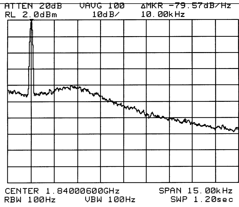
Figure 1 - Output Spectrum - Phase Noise
