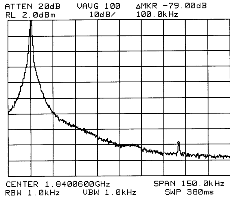
Figure 2 - Output Spectrum - Spurious
