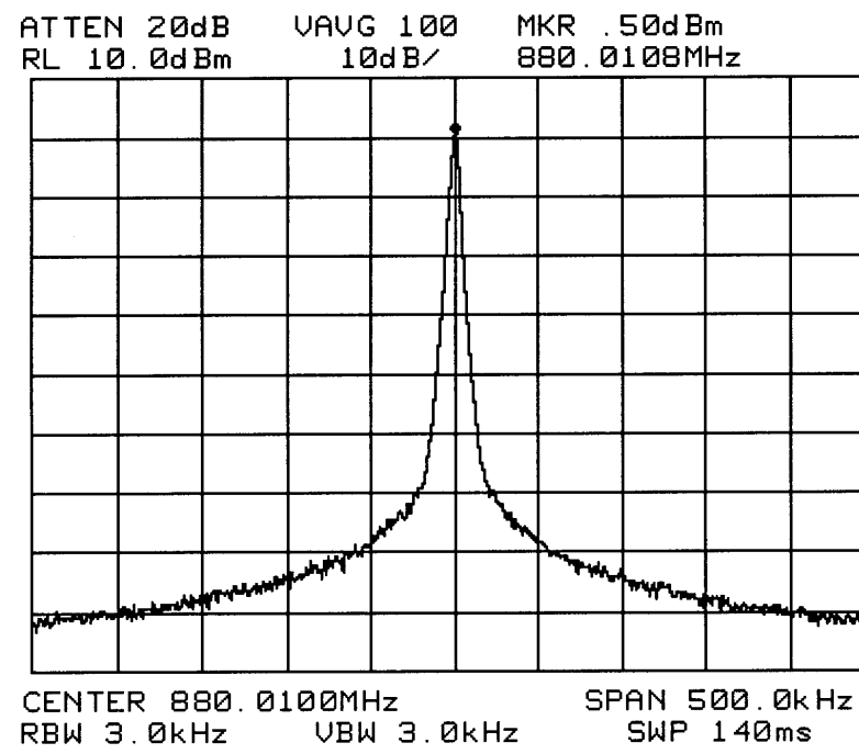
Figure 2 - Output Spectrum - Spurious
