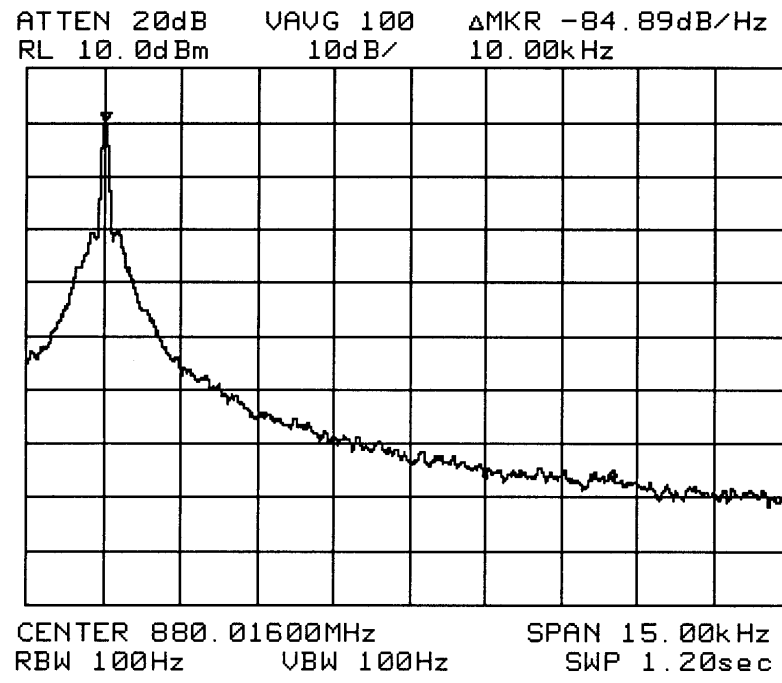
Figure 1 - Output Spectrum - Phase Noise (10kHz Step Size)
